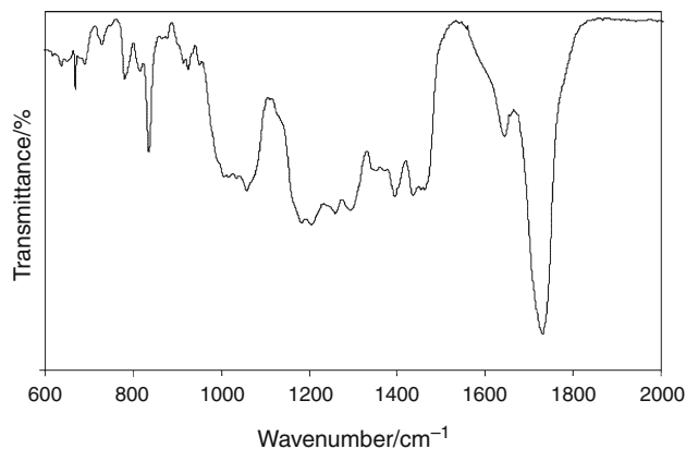
Fig. 2 Example FTIR spectra of novel epoxy-dicyclopentadiene-terminated polyesters
